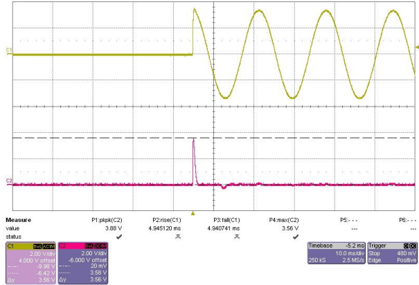
FS15-5 17.8A
